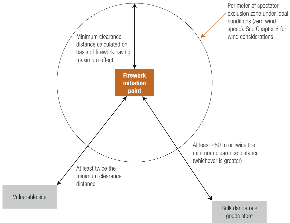
Figure 4.1 Example of set-up area showing minimum clearance distance, spectator exclusion zone and separation distances to facilities
