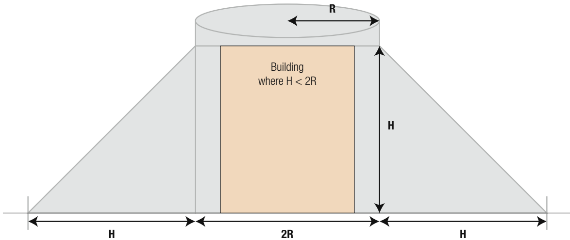
Figure 5.2 Side view showing exclusion zone for ground fireworks on a low building where H is less than 2R
