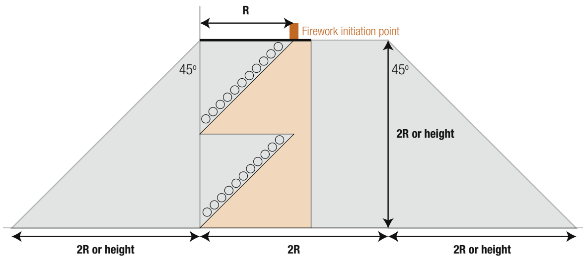
Figure 5.4 Side view showing exclusion zone for ground fireworks on a stadium
