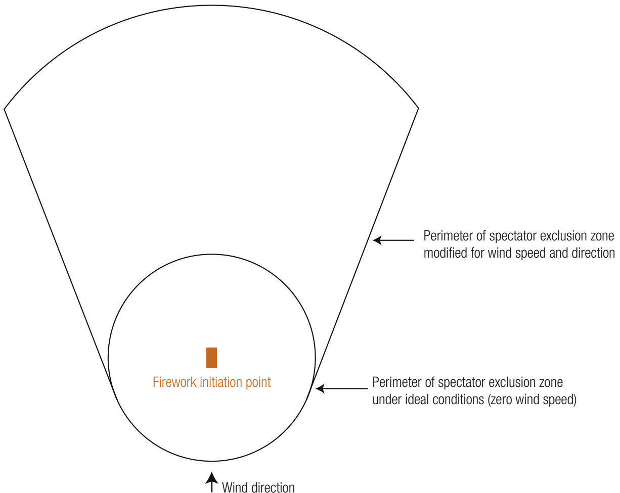
Figure 6.1 Example showing effect of wind on the spectator exclusion zone
