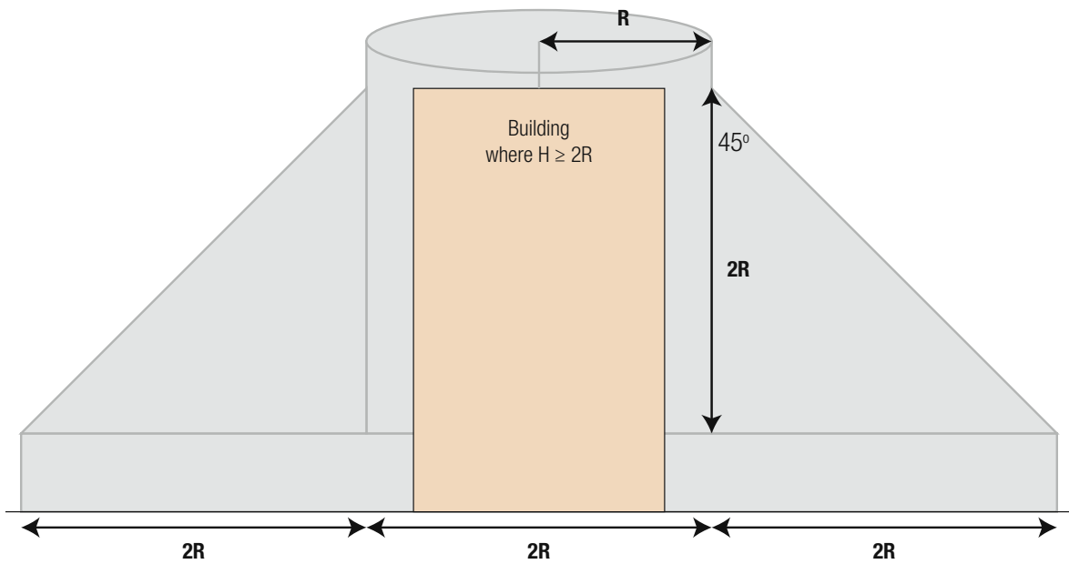
Figure 5.3 Side view showing exclusion zone for ground fireworks on a high building where H is 2R or more
